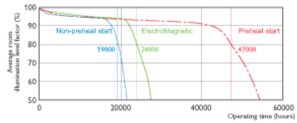
Service Life 3h cycle MASTER TL- D Xtra Polar
