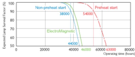
Life Expectancy 12h cycle MASTER TL- D Xtra Polar
