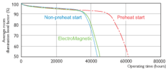
Service Life 12h cycle MASTER TL- D Xtra Polar
