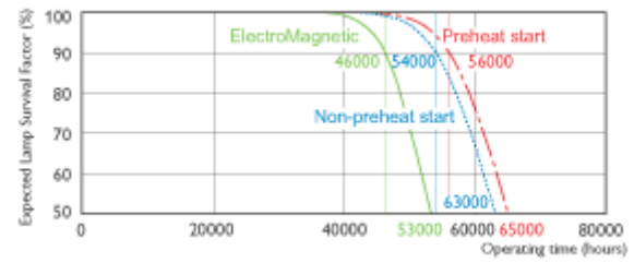
Life Expectancy 24h cycle MASTER TL- D Xtra Polar
