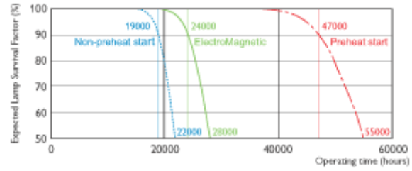
Life Expectancy 3h cycle MASTER TL- D Xtra Polar
