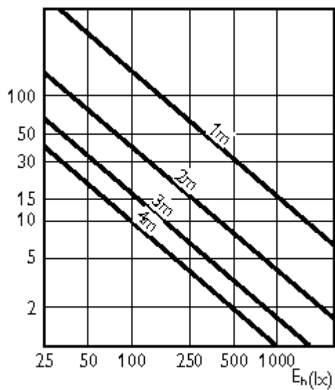
MASTERC CDM-R111 70W/830 24D
