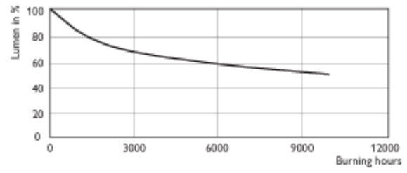
on electronic gear MASTERC CDM-R111 35W/830
