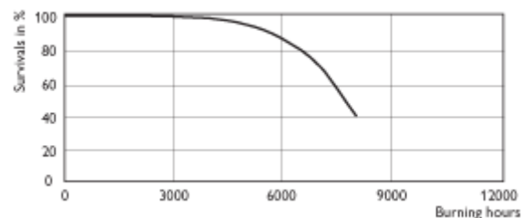
MASTERC CDM-R111 70W/830
