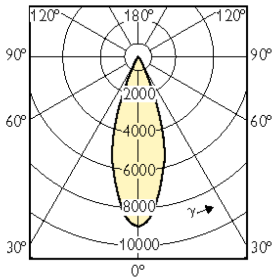
MASTERC CDM-R111 70W/830 40D
