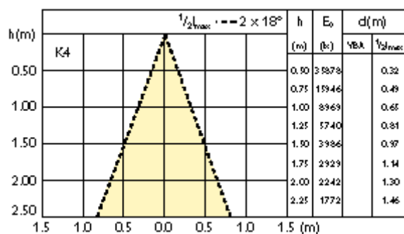
MASTERC CDM-R111 70W/830 40D
