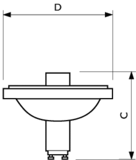
MASTERC CDM-R111 GX8.5
