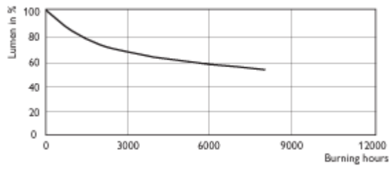
on electronic gear MASTERC CDM-R111 70W/830
