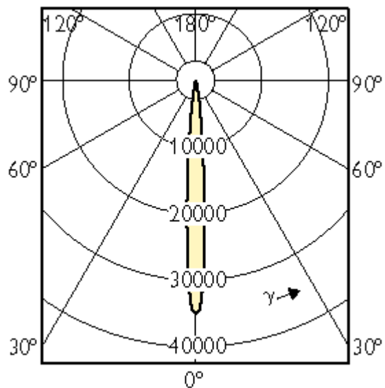
MASTERC CDM-R111 35W 10D
