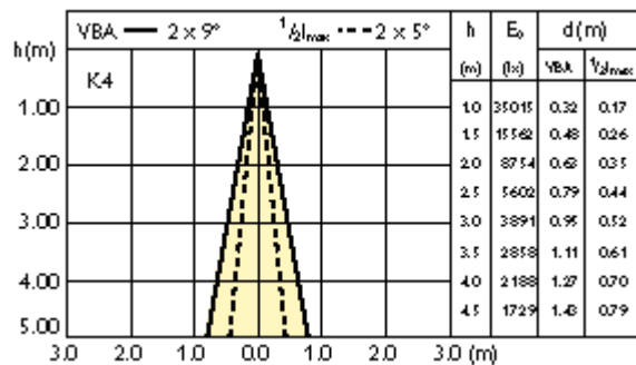
MASTERC CDM-R111 35W 10D
