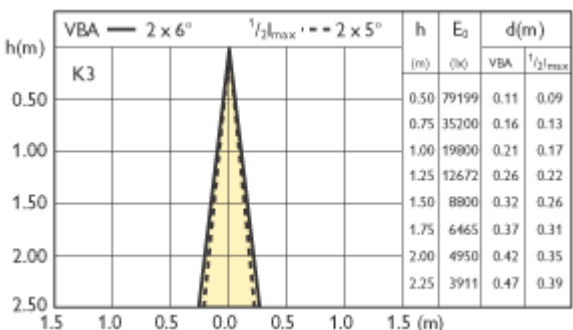
MASTERC CDM-R111 20W 10D
