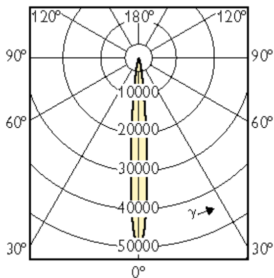
MASTERC CDM-R111 70W/830 10D
