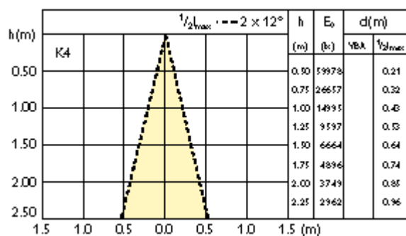
MASTERC CDM-R111 70W/830 24D
