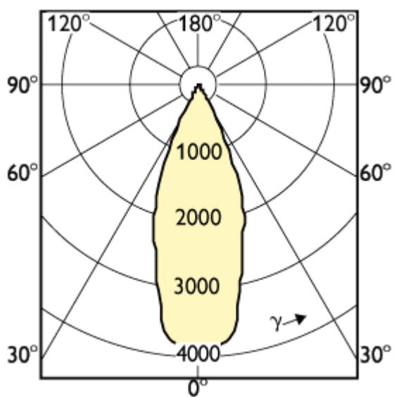
MASTERC CDM-R111 35W 40D
