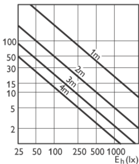
MASTERC CDM-R111 20W 10D
