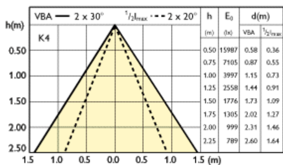
MASTERC CDM-R111 35W 40D
