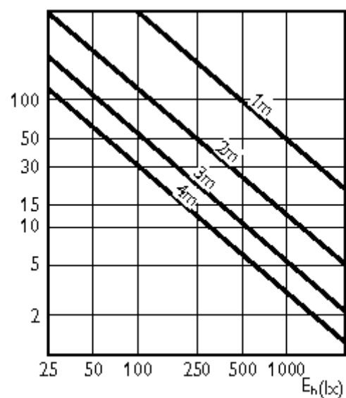
MASTERC CDM-R111 70W/830 10D
