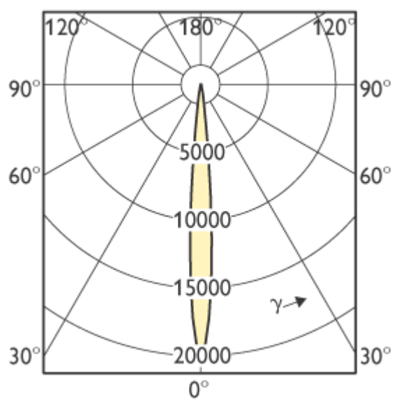
MASTERC CDM-R111 20W 10D
