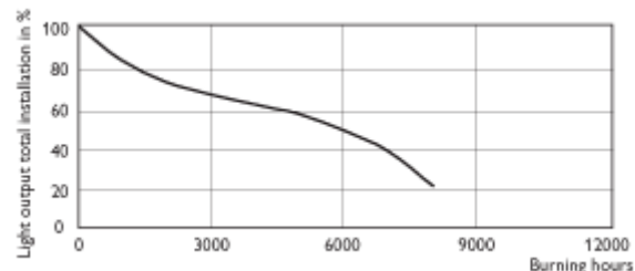
MASTERC CDM-R111 70W/830
