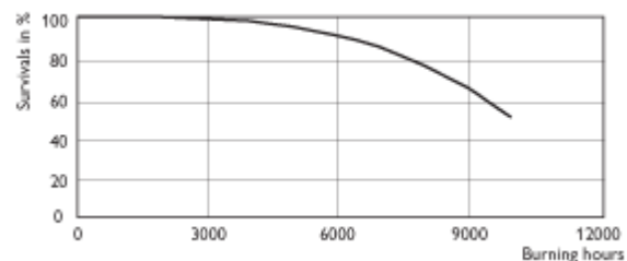
MASTERC CDM-R111 35W/830
