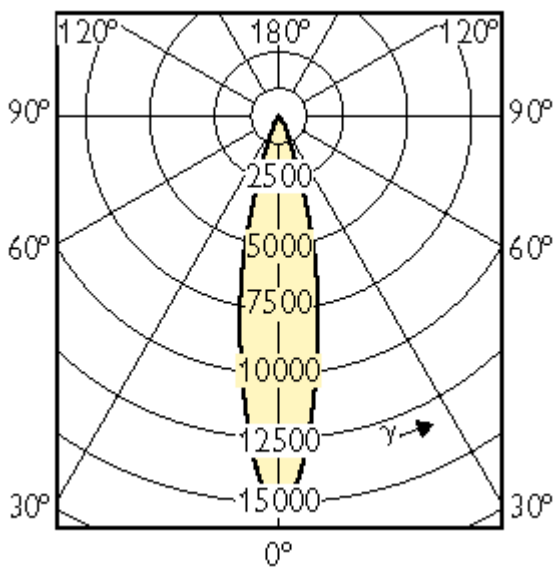
MASTERC CDM-R111 70W/830 24D
