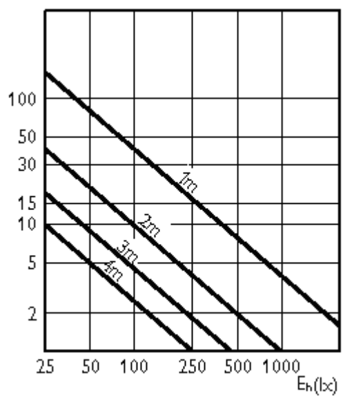
MASTERC CDM-R111 35W 40D
