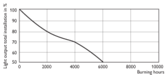
MASTERC CDM-TC 70W/830
