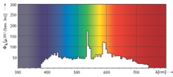
MASTERC CDM-TC 70W/942
