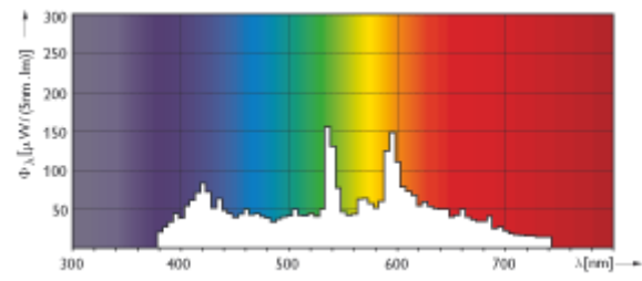
MASTERC CDM-TC 35W/942
