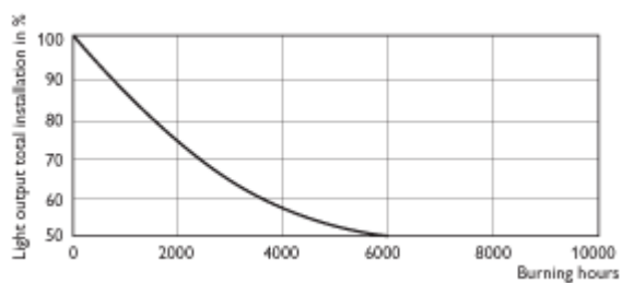
MASTERC CDM-TC 35W/830
