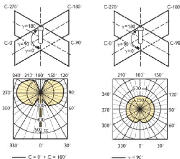
MASTERC CDM-TC 35W/830
