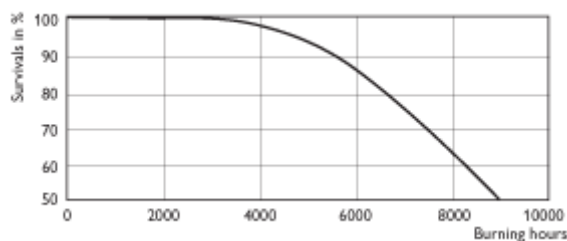
MASTERC CDM-TC 35W/830
