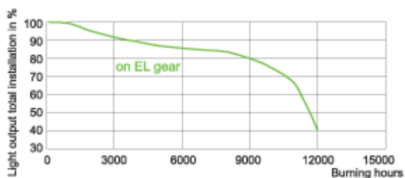
on electronic gear MASTERC CDM-T Elite 70W/930
