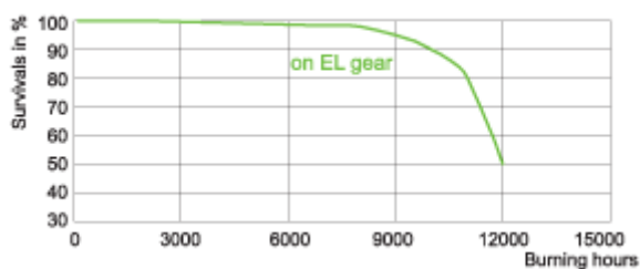
on electronic gear MASTERC CDM-T Elite 150W/930
