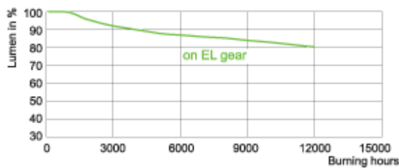
on electronic gear MASTERC CDM-T Elite 70W/930
