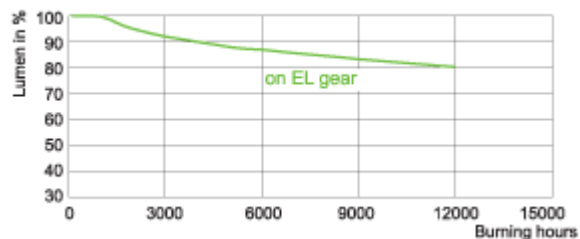
on electronic gear MASTERC CDM-T Elite 150W/930
