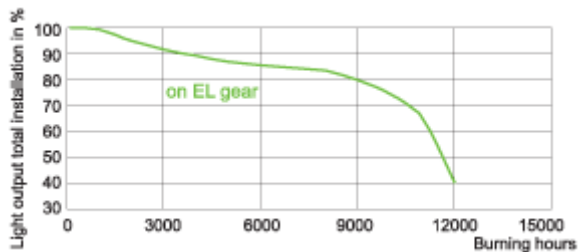
on electronic gear MASTERC CDM-T Elite 35W/930
