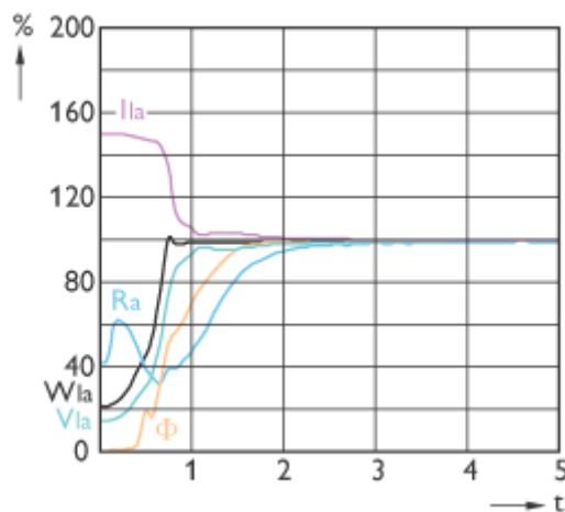
MASTERC CDM-T Elite 70W/930
