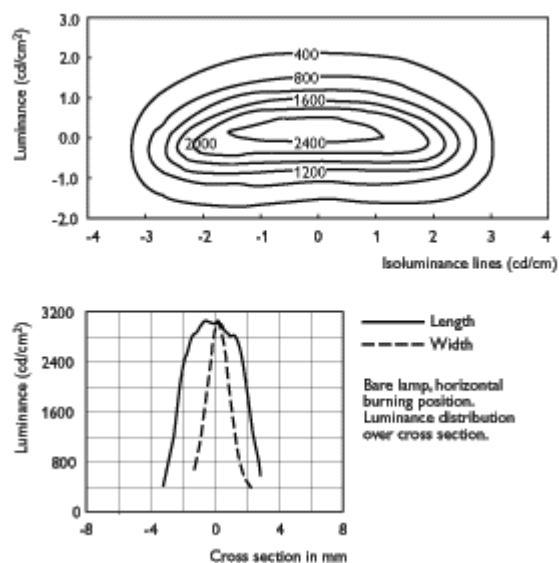
MASTERC CDM-T Elite 35W
