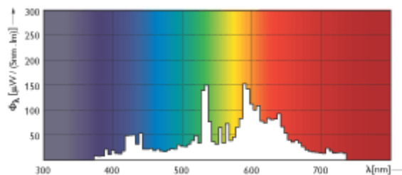
MASTERColour CDM-T Elite 150W /930 MASTERC CDM-T Elite 150W/930
