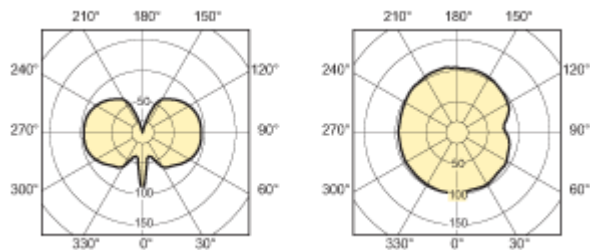
MASTERC CDM-T Elite 70W/930
