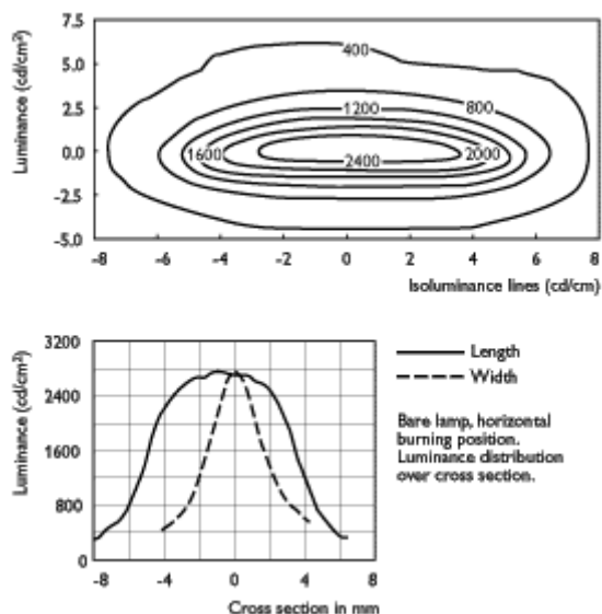
MASTERC CDM-T Elite 150W
