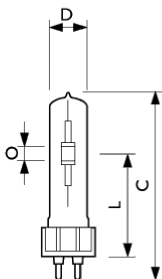
MASTERC CDM-T Elite 100W/150W/250W/35W/70W
