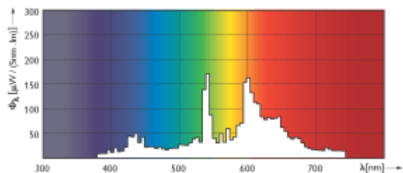
MASTERColour CDM-T Elite 70W /930 MASTERC CDM-T Elite 70W/930
