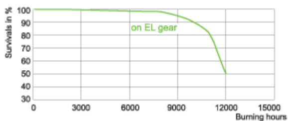
on electronic gear MASTERC CDM-T Elite 35W/930
