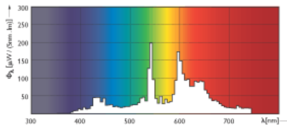
MASTERColour CDM-T Elite 35W /930 MASTERC CDM-T Elite 35W/930
