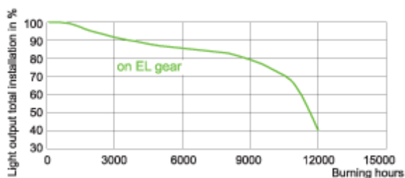
on electronic gear MASTERC CDM-T Elite 150W/930
