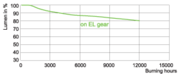
on electronic gear MASTERC CDM-T Elite 35W/930
