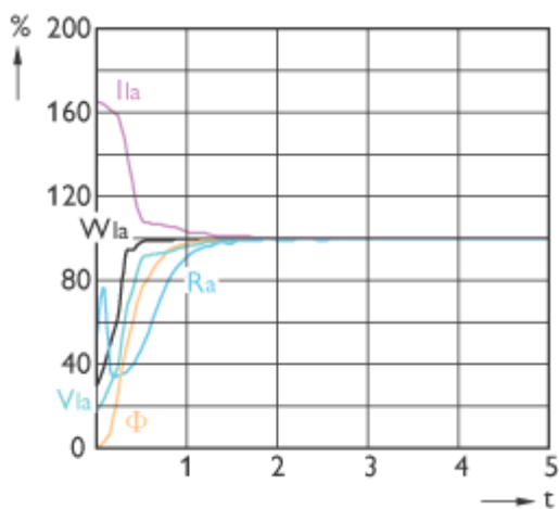
MASTERC CDM-T Elite 35W/930
