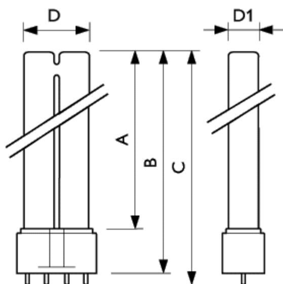
MASTER PL- L Xtra
