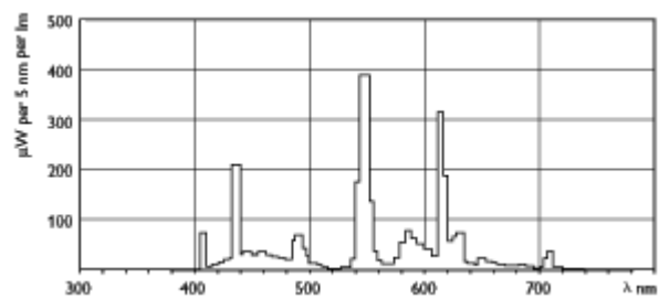
MASTER PL-L Xtra/840
