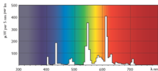
MASTER PL-L Xtra/830
