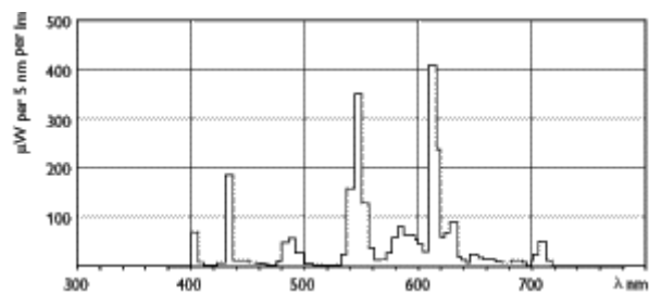
MASTER PL-L Xtra/830
