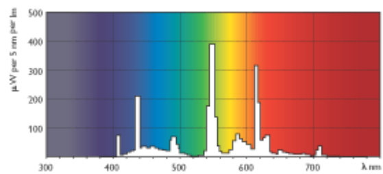
MASTER PL-L Xtra/840
