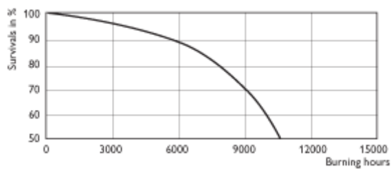
MHN- TD 70W/150W/842
