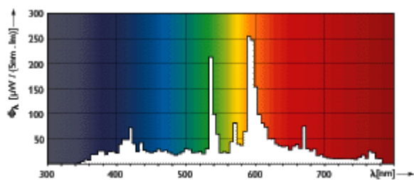
MHN- TD 150W/70W
