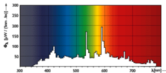
MHN- TD 150W/70W
