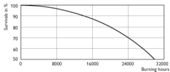
SON 100W/150W/250W/400W
