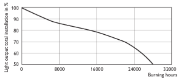
SON 100W/150W/250W/400W
